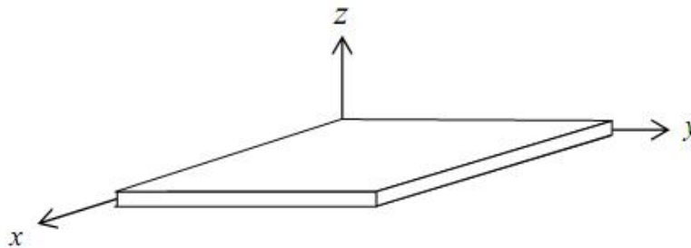
Fig.4: Cartesian axes
